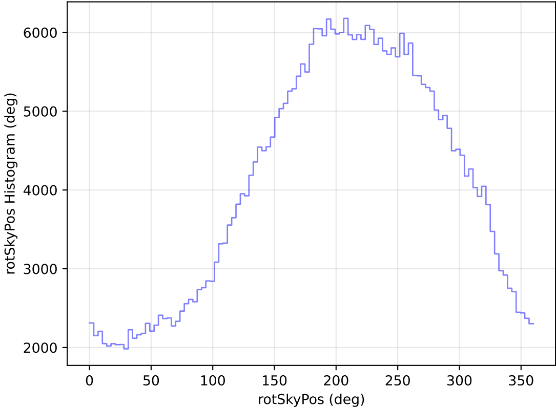
internal_u_expt60_nscale1.1v3.4_10yrs WFD z band: rotSkyPos Histogram
