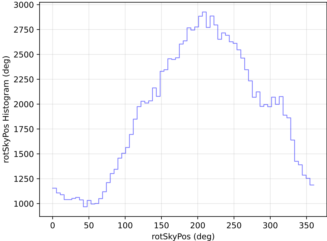
internal_u_expt60_nscale1.1v3.4_10yrs WFD u band: rotSkyPos Histogram
