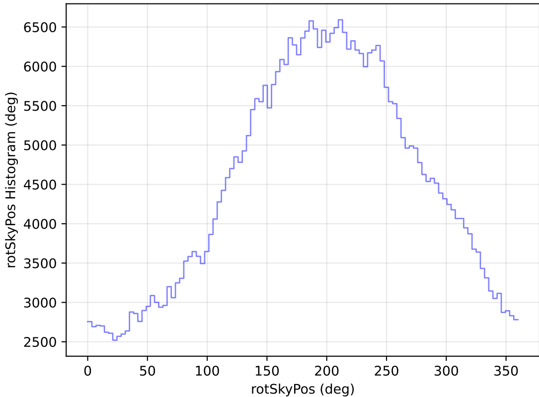
internal_u_expt60_nscale1.1v3.4_10yrs WFD r band: rotSkyPos Histogram
