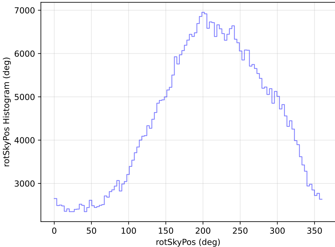
internal_u_expt60_nscale1.1v3.4_10yrs WFD i band: rotSkyPos Histogram
