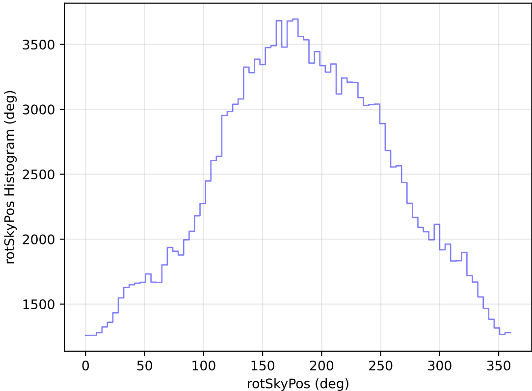
internal_u_expt60_nscale1.1v3.4_10yrs WFD g band: rotSkyPos Histogram
