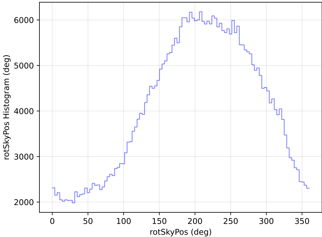
internal_u_expt60_nscale1.1v3.4_10yrs All sky z band: rotSkyPos Histogram
