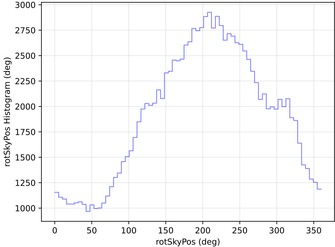
internal_u_expt60_nscale1.1v3.4_10yrs All sky u band: rotSkyPos Histogram
