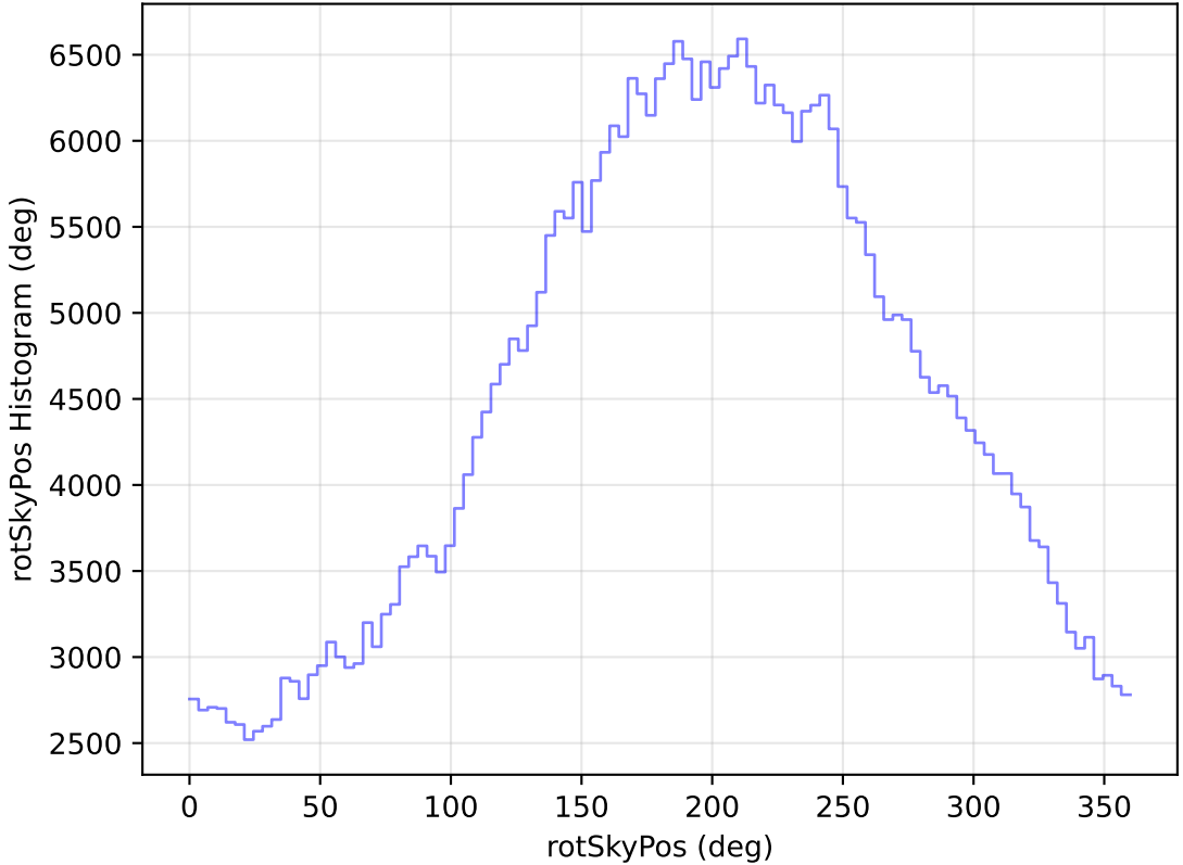
internal_u_expt60_nscale1.1v3.4_10yrs All sky r band: rotSkyPos Histogram
