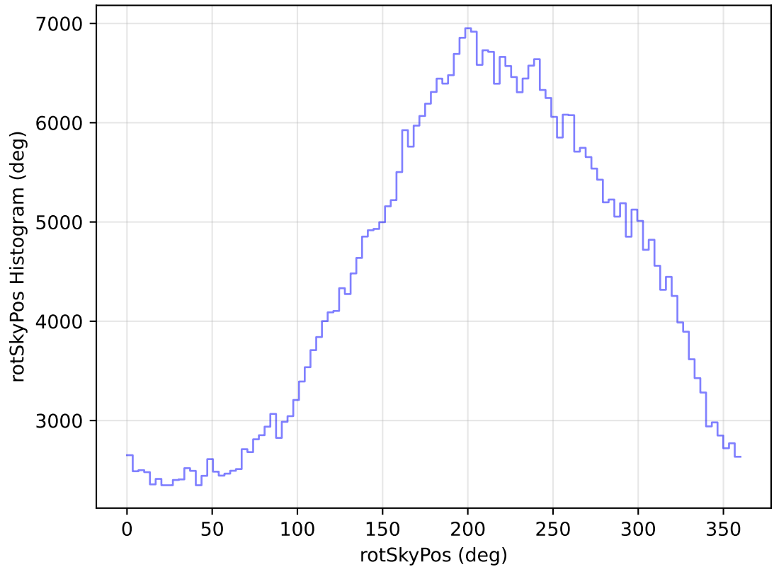
internal_u_expt60_nscale1.1v3.4_10yrs All sky i band: rotSkyPos Histogram
