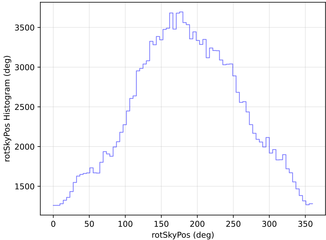
internal_u_expt60_nscale1.1v3.4_10yrs All sky g band: rotSkyPos Histogram
