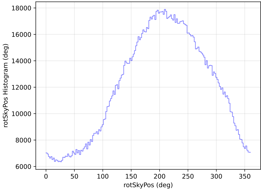
internal_u_expt60_nscale1.1v3.4_10yrs All sky all bands: rotSkyPos Histogram
