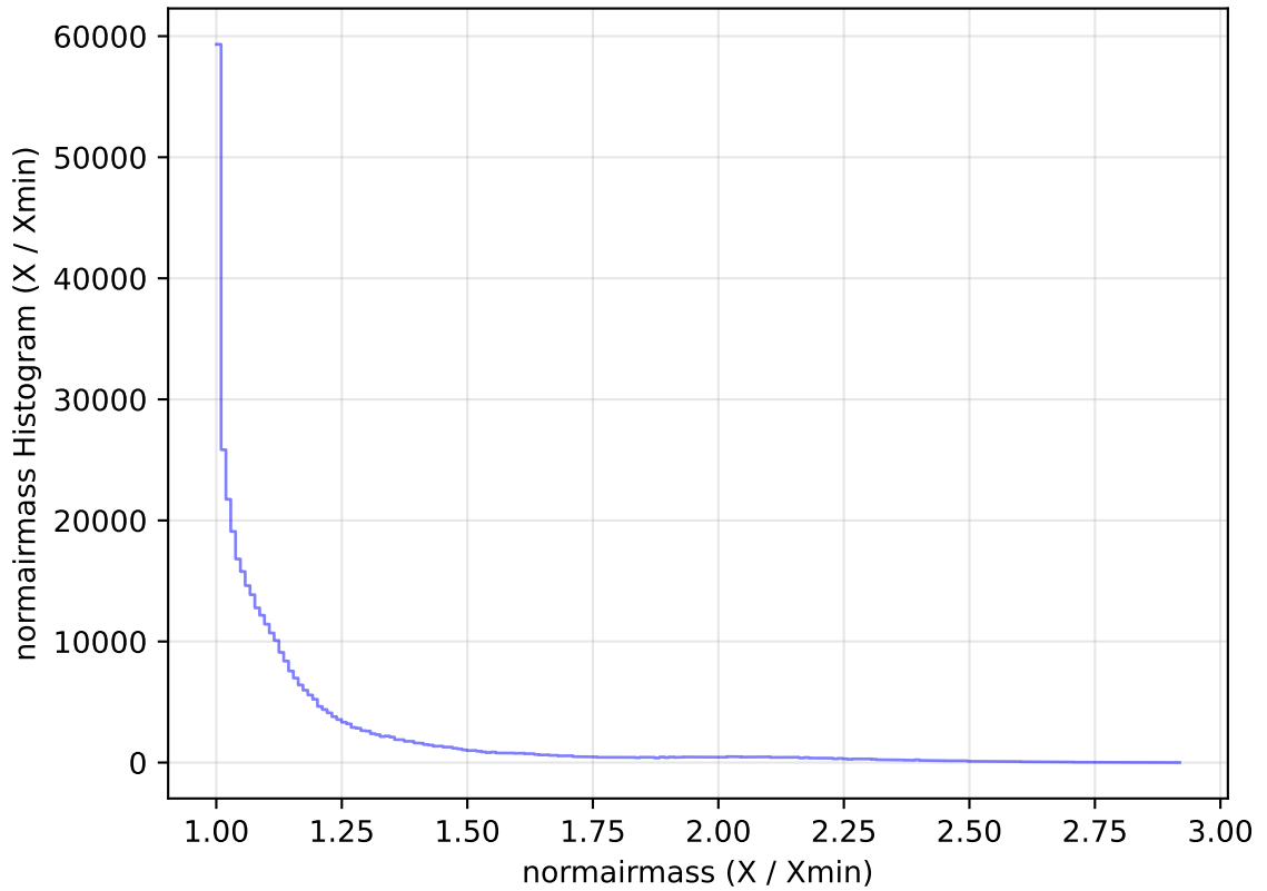
internal_u_expt60_nscale1.1v3.4_10yrs WFD z band: normairmass Histogram
