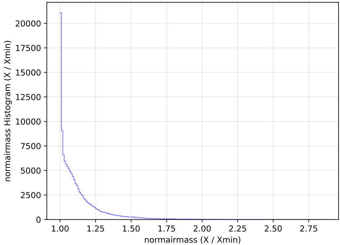
internal_u_expt60_nscale1.1v3.4_10yrs WFD u band: normairmass Histogram
