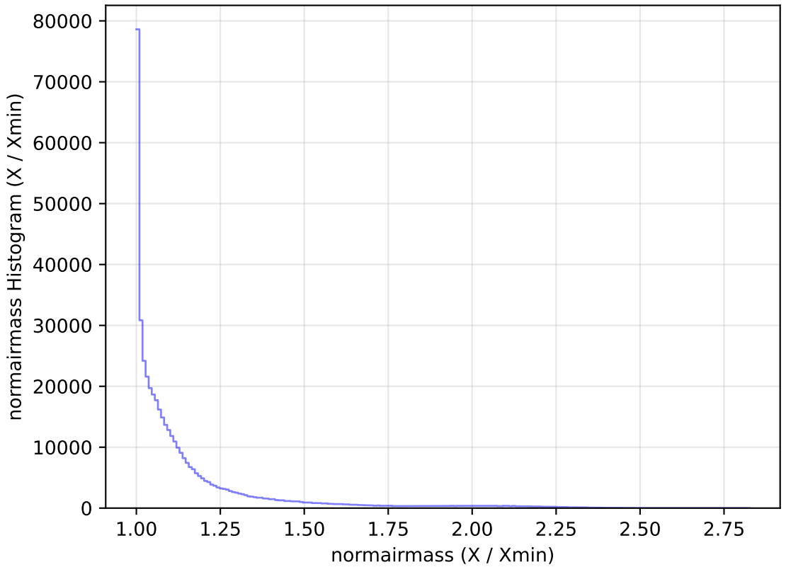
internal_u_expt60_nscale1.1v3.4_10yrs WFD r band: normairmass Histogram
