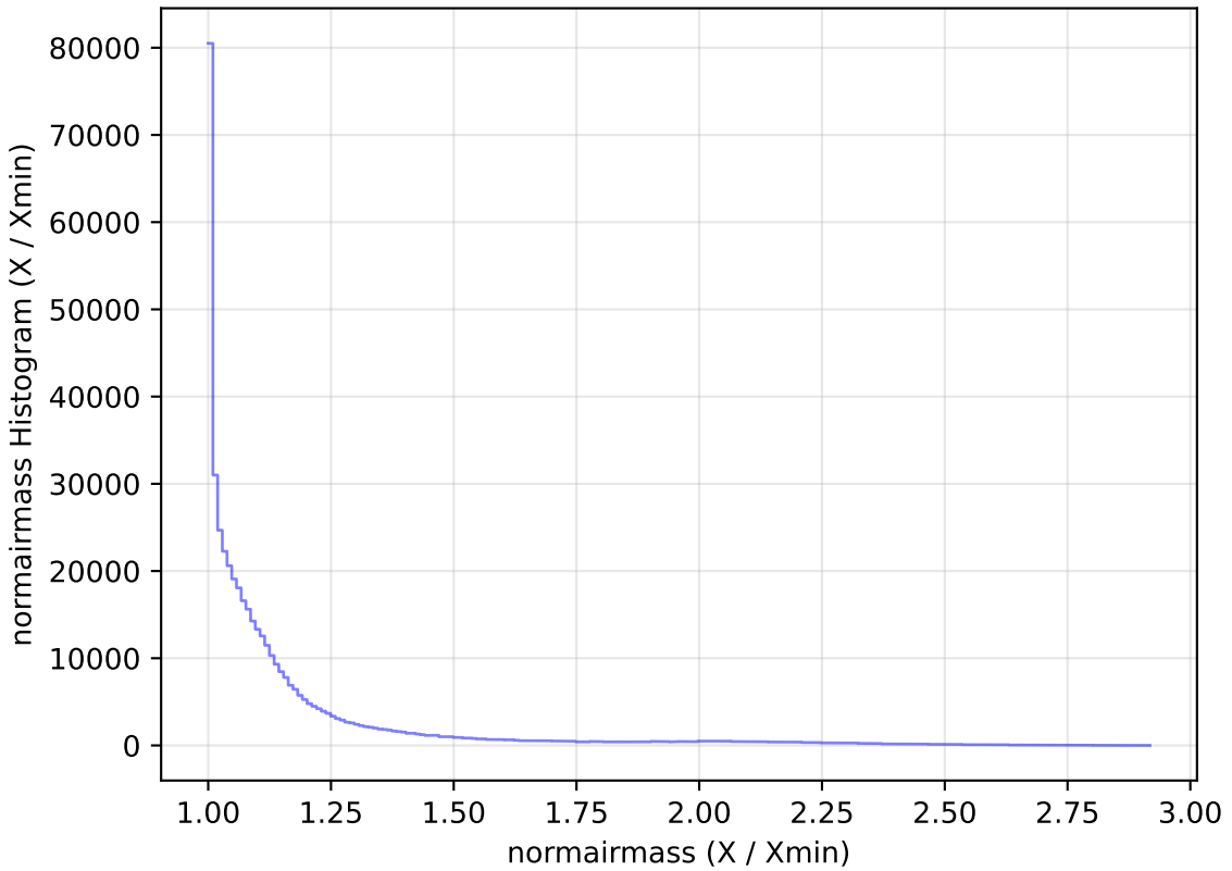
internal_u_expt60_nscale1.1v3.4_10yrs WFD i band: normairmass Histogram
