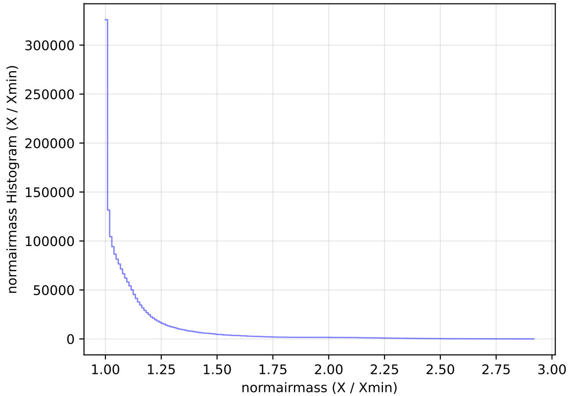
internal_u_expt60_nscale1.1v3.4_10yrs WFD all bands: normairmass Histogram
