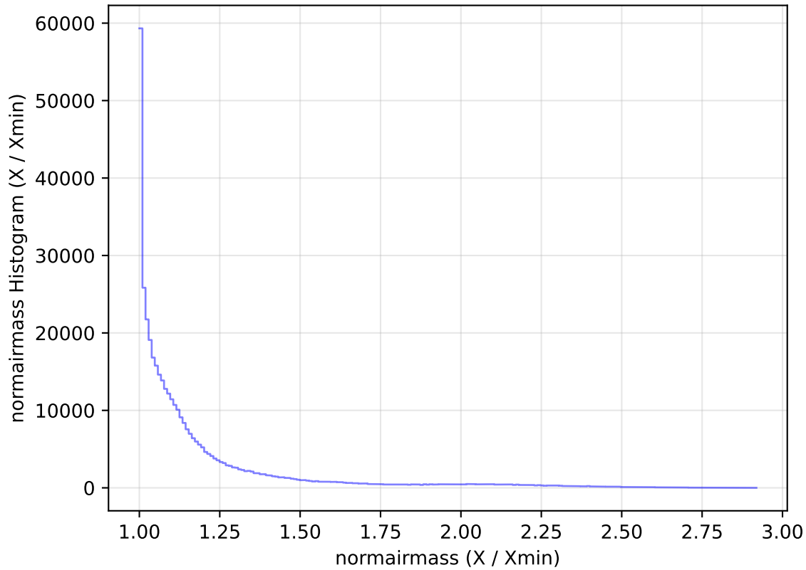
internal_u_expt60_nscale1.1v3.4_10yrs All sky z band: normairmass Histogram
