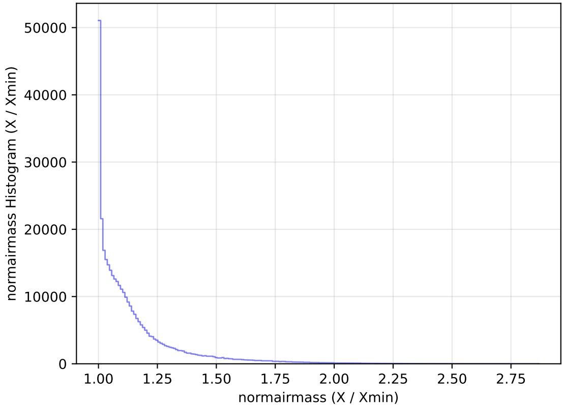
internal_u_expt60_nscale1.1v3.4_10yrs All sky y band: normairmass Histogram
