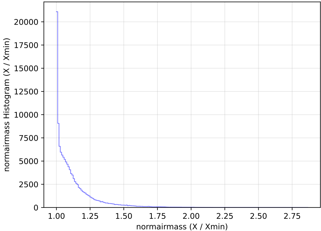
internal_u_expt60_nscale1.1v3.4_10yrs All sky u band: normairmass Histogram
