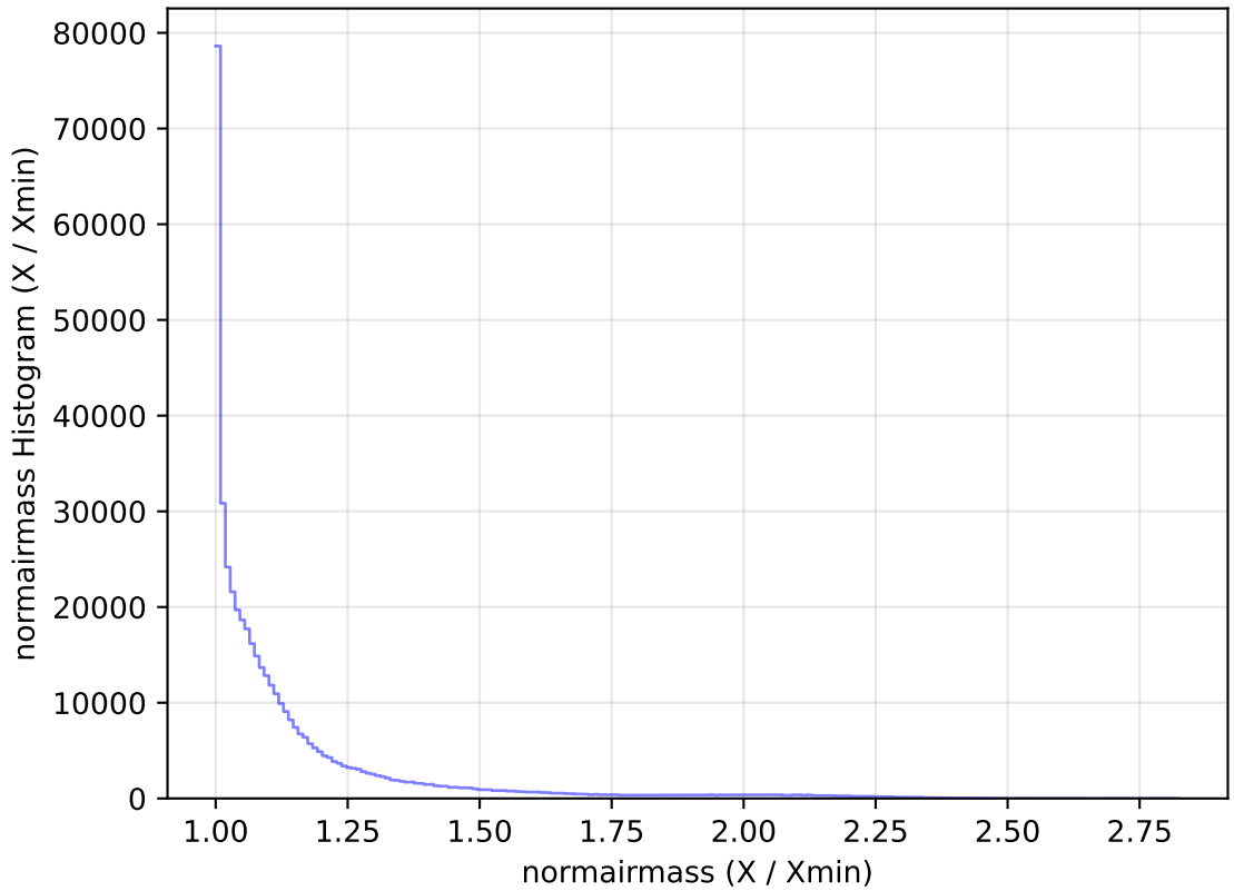
internal_u_expt60_nscale1.1v3.4_10yrs All sky r band: normairmass Histogram
