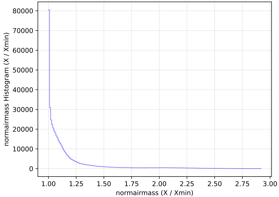
internal_u_expt60_nscale1.1v3.4_10yrs All sky i band: normairmass Histogram
