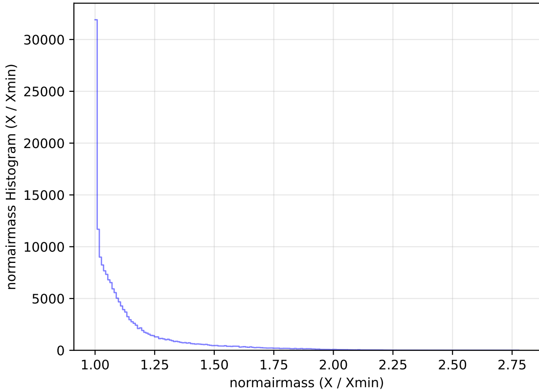
internal_u_expt60_nscale1.1v3.4_10yrs All sky g band: normairmass Histogram
