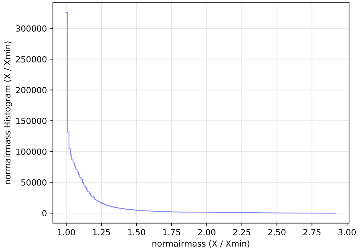
internal_u_expt60_nscale1.1v3.4_10yrs All sky all bands: normairmass Histogram
