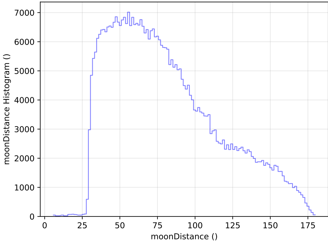
internal_u_expt60_nscale1.1v3.4_10yrs WFD z band: moonDistance Histogram
