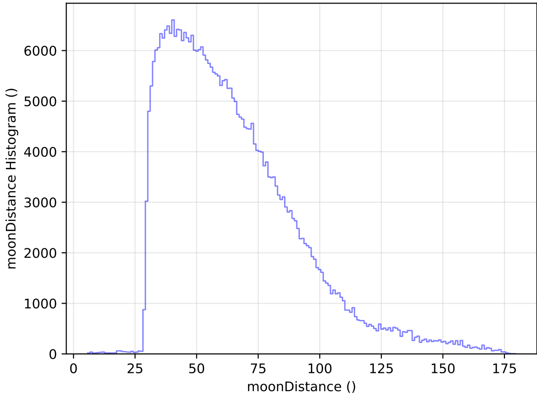
internal_u_expt60_nscale1.1v3.4_10yrs WFD y band: moonDistance Histogram
