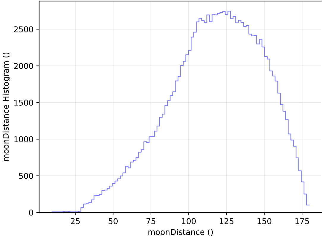
internal_u_expt60_nscale1.1v3.4_10yrs WFD u band: moonDistance Histogram
