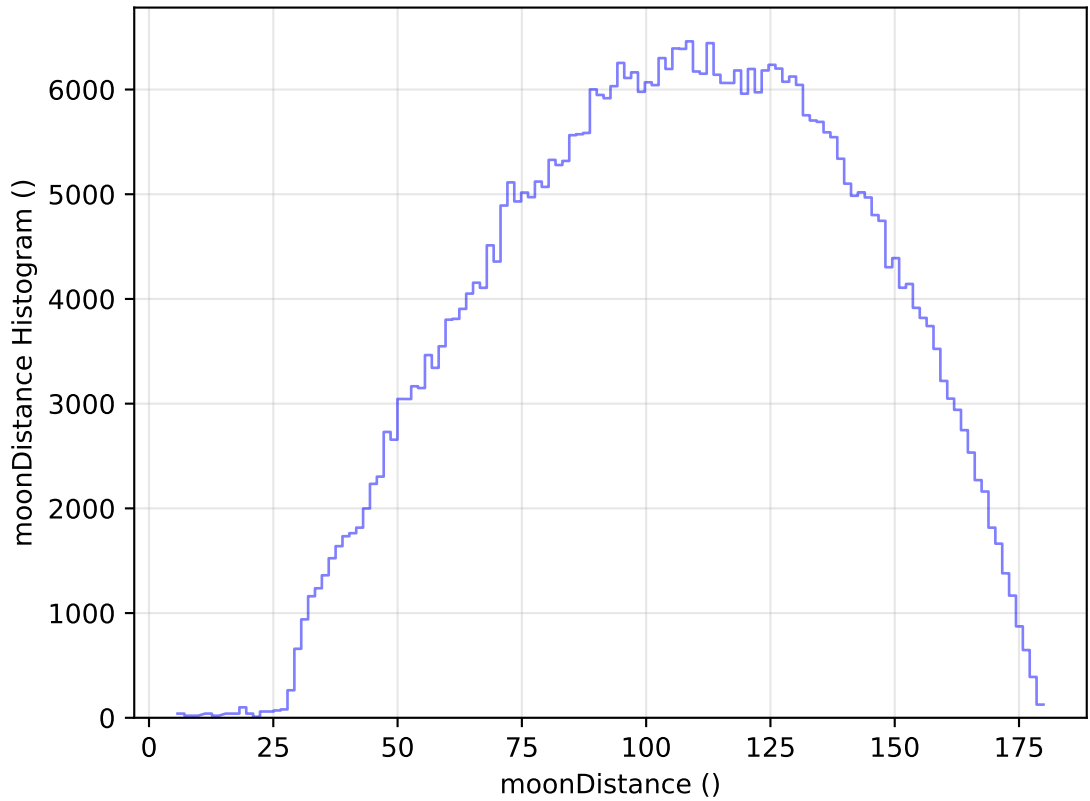
internal_u_expt60_nscale1.1v3.4_10yrs WFD r band: moonDistance Histogram
