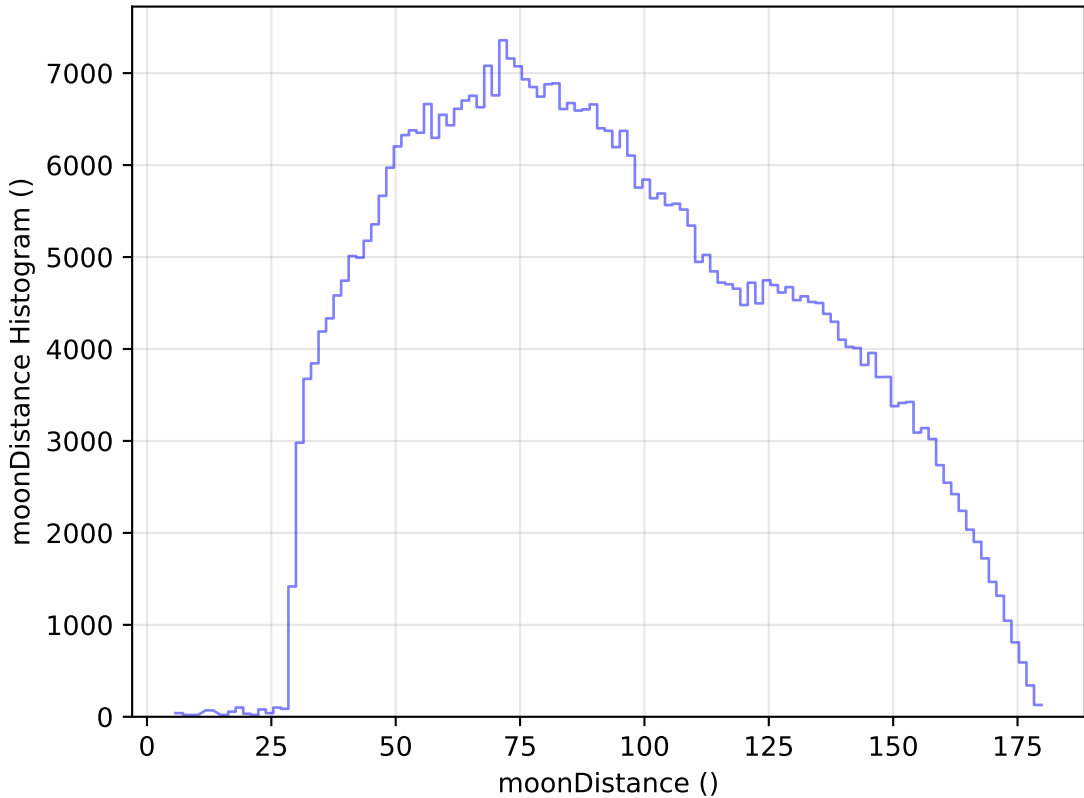
internal_u_expt60_nscale1.1v3.4_10yrs WFD i band: moonDistance Histogram
