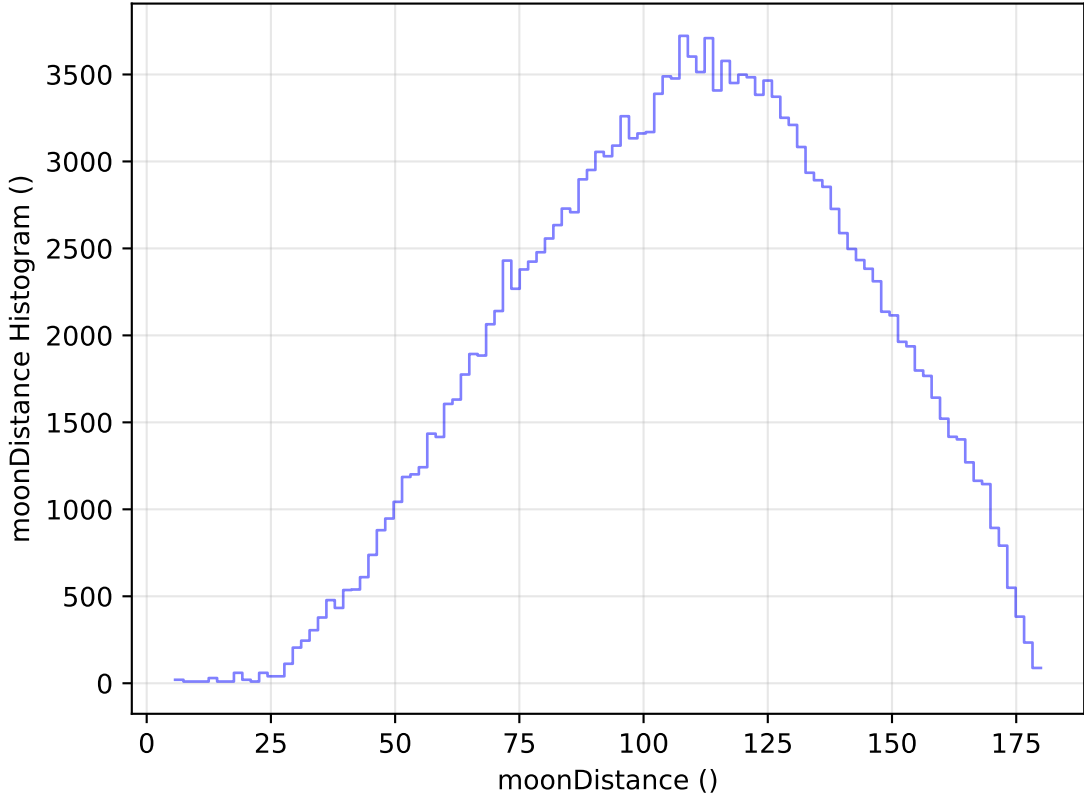
internal_u_expt60_nscale1.1v3.4_10yrs WFD g band: moonDistance Histogram
