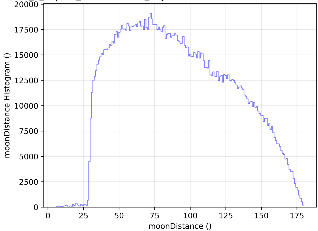
internal_u_expt60_nscale1.1v3.4_10yrs WFD all bands: moonDistance Histogram
