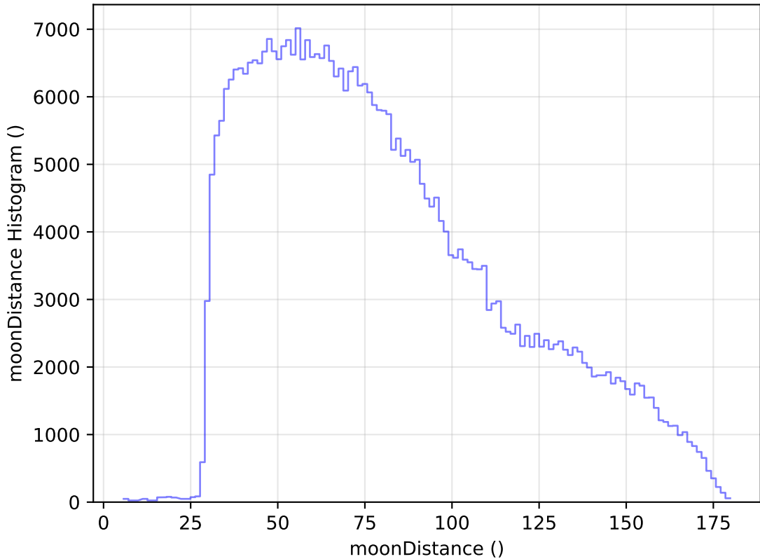
internal_u_expt60_nscale1.1v3.4_10yrs All sky z band: moonDistance Histogram
