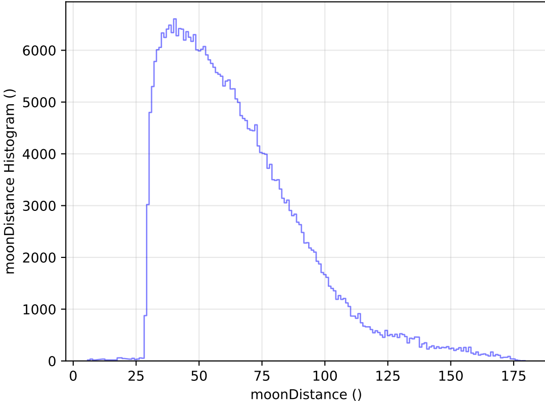
internal_u_expt60_nscale1.1v3.4_10yrs All sky y band: moonDistance Histogram
