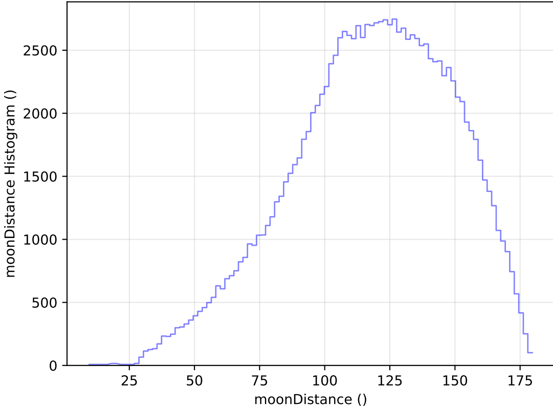
internal_u_expt60_nscale1.1v3.4_10yrs All sky u band: moonDistance Histogram
