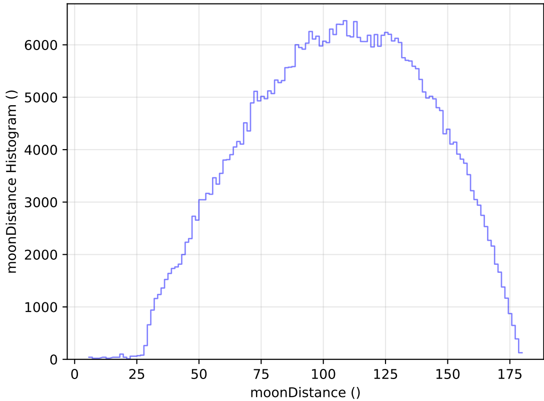
internal_u_expt60_nscale1.1v3.4_10yrs All sky r band: moonDistance Histogram
