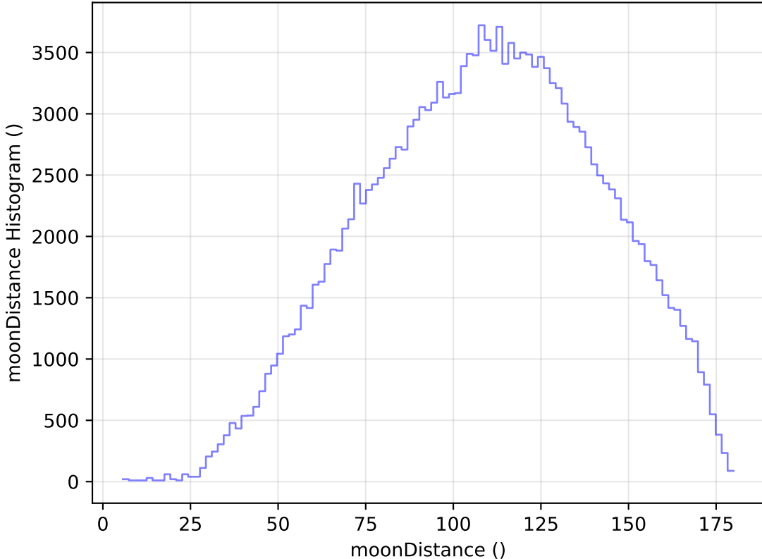
internal_u_expt60_nscale1.1v3.4_10yrs All sky g band: moonDistance Histogram
