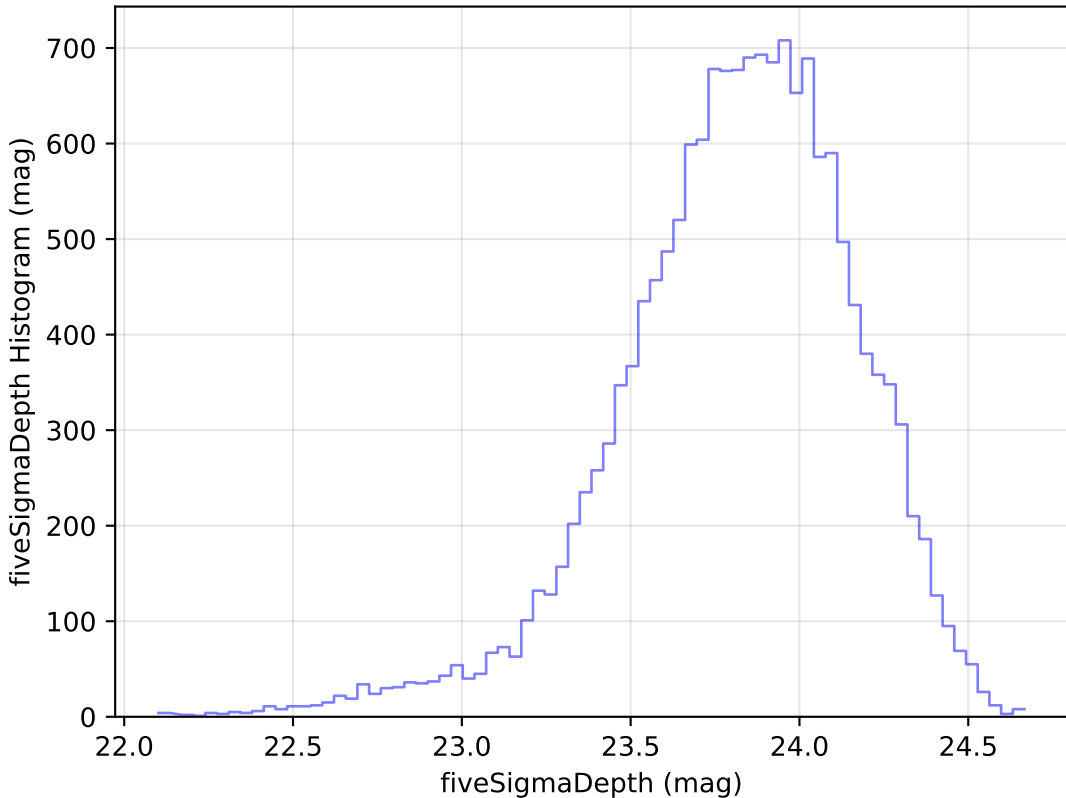
internal_u_expt60_nscale1.1v3.4_10yrs Yr 1 u band: fiveSigmaDepth Histogram
