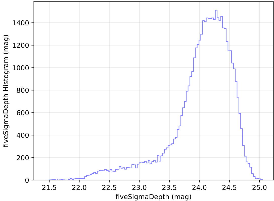
internal_u_expt60_nscale1.1v3.4_10yrs Yr 1 r band: fiveSigmaDepth Histogram
