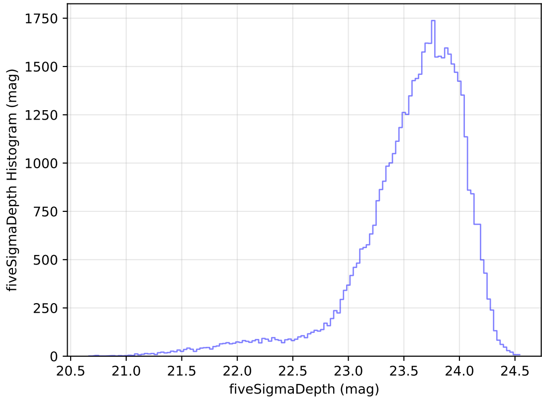
internal_u_expt60_nscale1.1v3.4_10yrs Yr 1 i band: fiveSigmaDepth Histogram
