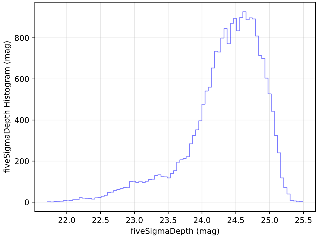
internal_u_expt60_nscale1.1v3.4_10yrs Yr 1 g band: fiveSigmaDepth Histogram
