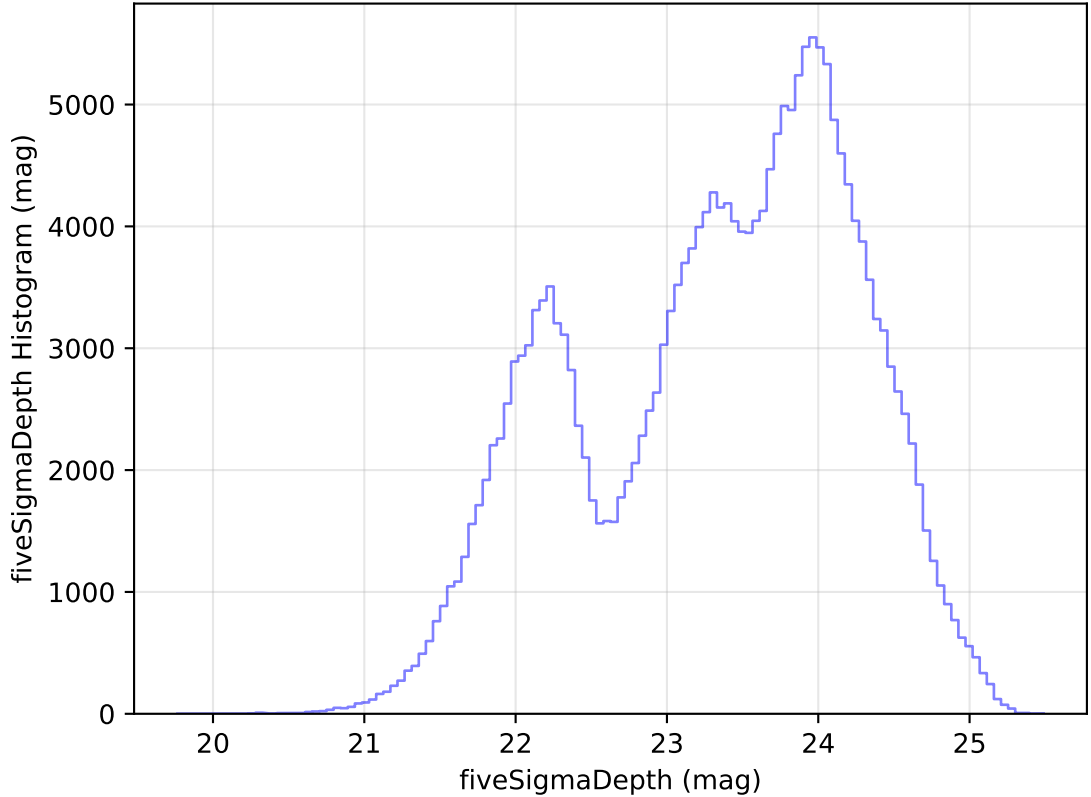
internal_u_expt60_nscale1.1v3.4_10yrs Yr 1 all bands: fiveSigmaDepth Histogram
