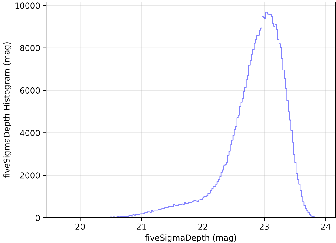
internal_u_expt60_nscale1.1v3.4_10yrs WFD z band: fiveSigmaDepth Histogram
