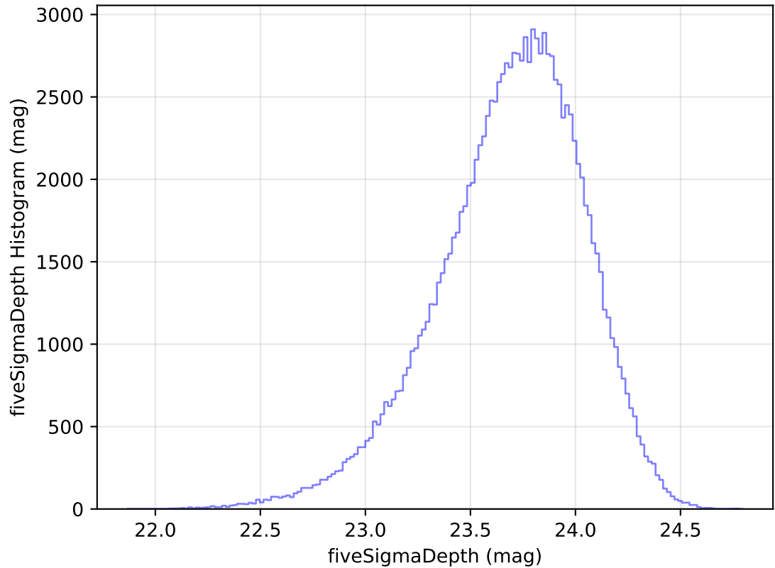
internal_u_expt60_nscale1.1v3.4_10yrs WFD u band: fiveSigmaDepth Histogram
