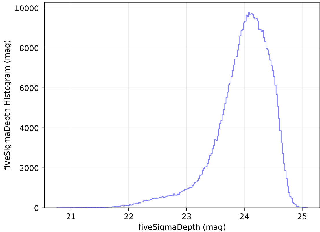
internal_u_expt60_nscale1.1v3.4_10yrs WFD r band: fiveSigmaDepth Histogram
