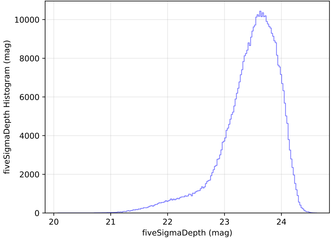
internal_u_expt60_nscale1.1v3.4_10yrs WFD i band: fiveSigmaDepth Histogram
