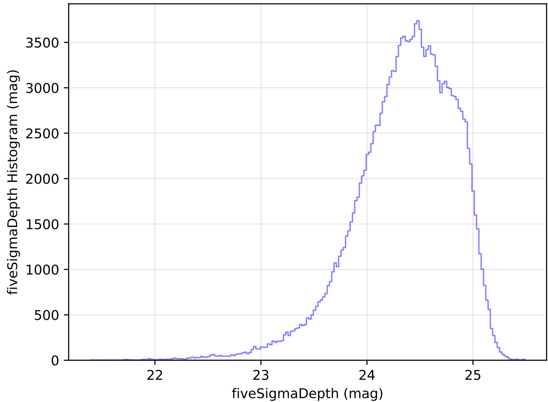
internal_u_expt60_nscale1.1v3.4_10yrs WFD g band: fiveSigmaDepth Histogram
