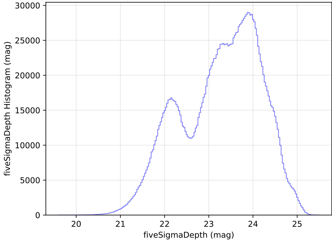
internal_u_expt60_nscale1.1v3.4_10yrs WFD all bands: fiveSigmaDepth Histogram
