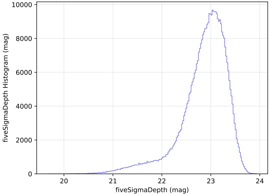
internal_u_expt60_nscale1.1v3.4_10yrs All sky z band: fiveSigmaDepth Histogram
