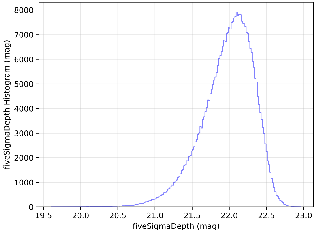
internal_u_expt60_nscale1.1v3.4_10yrs All sky y band: fiveSigmaDepth Histogram
