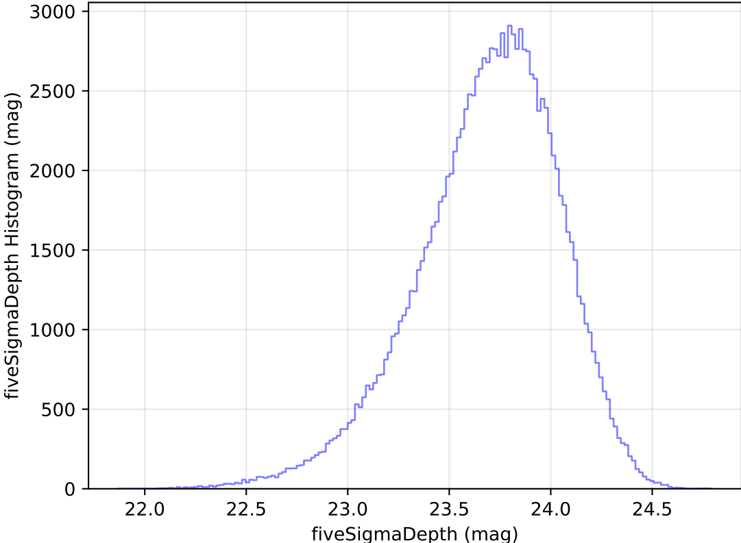
internal_u_expt60_nscale1.1v3.4_10yrs All sky u band: fiveSigmaDepth Histogram
