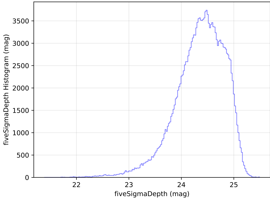
internal_u_expt60_nscale1.1v3.4_10yrs All sky g band: fiveSigmaDepth Histogram
